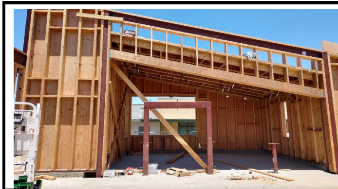
Framing at Building C
